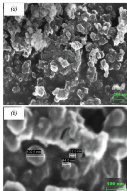
Fig. 4. SEM images of (L-NS3) produced by continued method (a–b).
